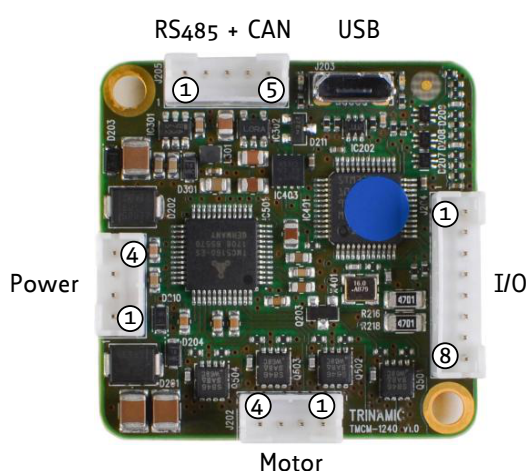
Figure 2: PD42-x-1240 connectors
