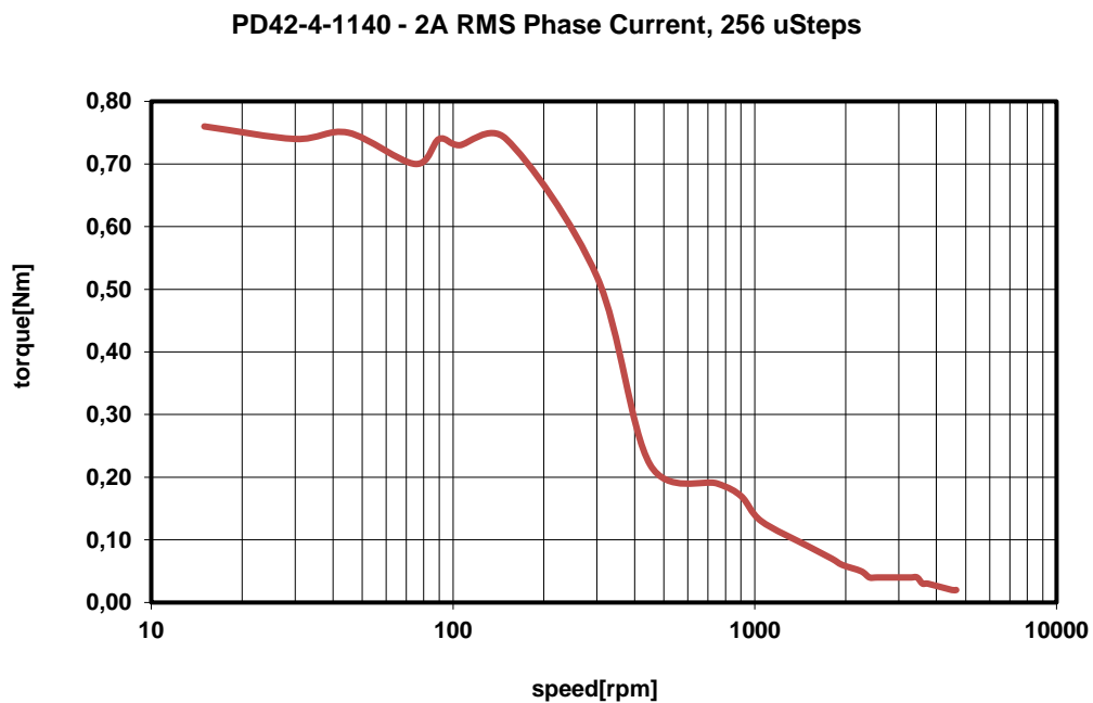
Figure 9.4 PD42-4-1140 torque vs. velocity 24V / 2A, 256 \mu steps
