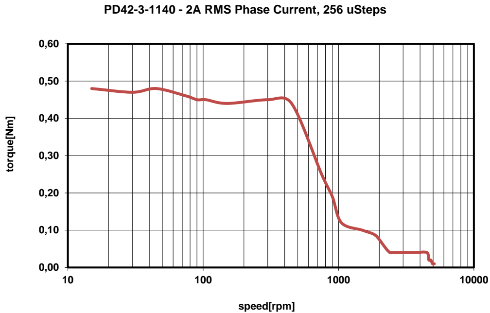
Figure 9.3 PD42-3-1140 torque vs. velocity 24V / 2A, 256 \mu steps
