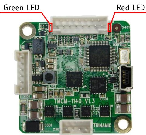
Figure 7.1 On-board LEDs
