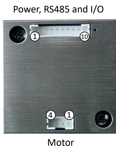
Figure 2: PD42-x-1370 connectors
