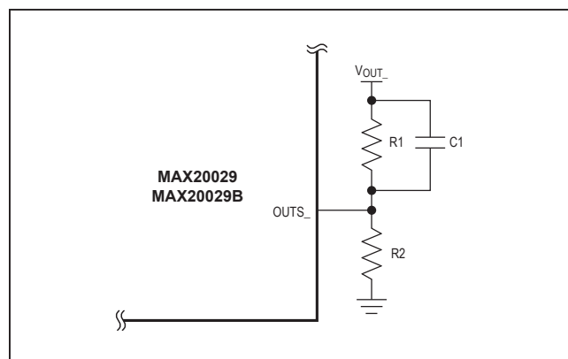
Figure 4. Adjustable Output-Voltage Configuration
