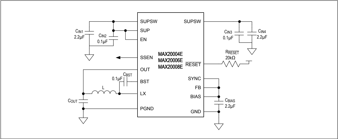
Typical Application Circuit for f_{SW} = 2.1\text{MHz} , I_{OUT} = 6\text{A} and Fixed Output Voltage Version
