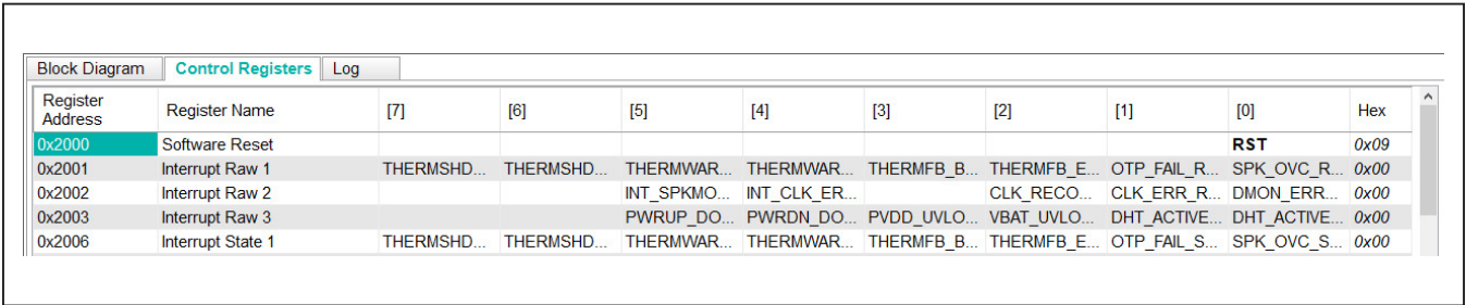
Figure 6. Control Register Tab
