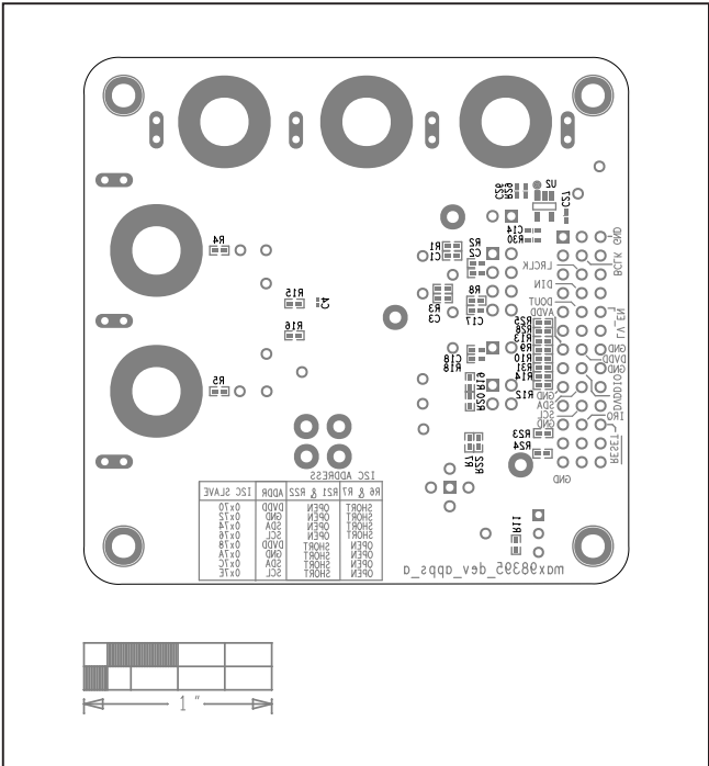
MAX98395 EV System Component Placement Guide—Bottom Silkscreen
