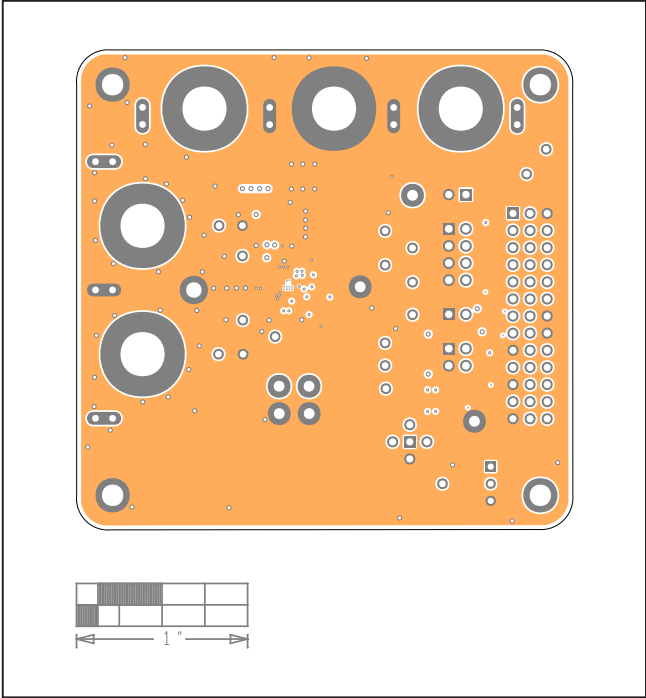
MAX98395 EV System PCB Layout—GND L5
