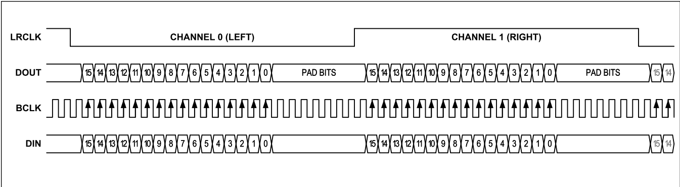
Figure 1. Standard I²S Mode
