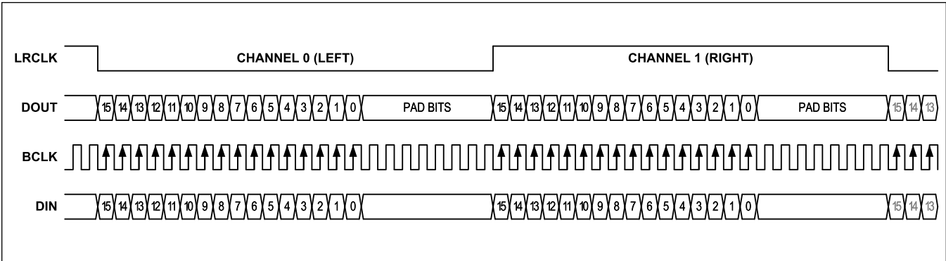
Figure 2. Left-Justified Mode
