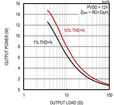
OUTPUT POWER vs. LOAD IMPEDANCE toc36
