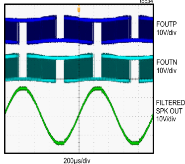
CLIPPING RESPONSE FOR 1% TOTAL HARMONIC DISTORTION PLUS NOISE toc34
