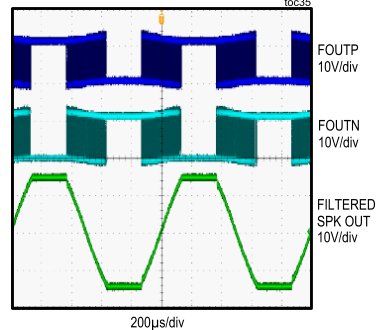
CLIPPING RESPONSE FOR 10% TOTAL HARMONIC DISTORTION PLUS NOISE toc35
