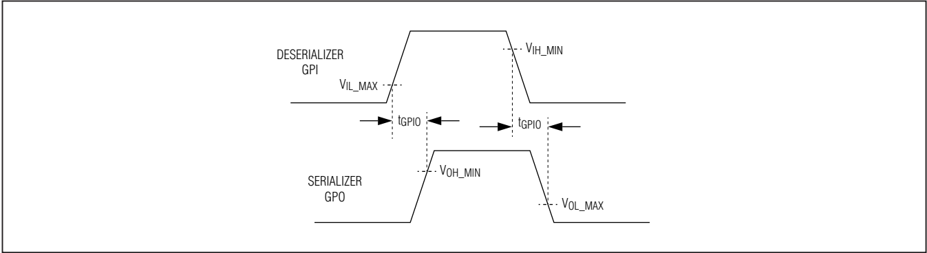
Figure 9. GPI-to-GPO Delay
