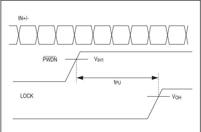
Figure 11. Power-Up Delay
