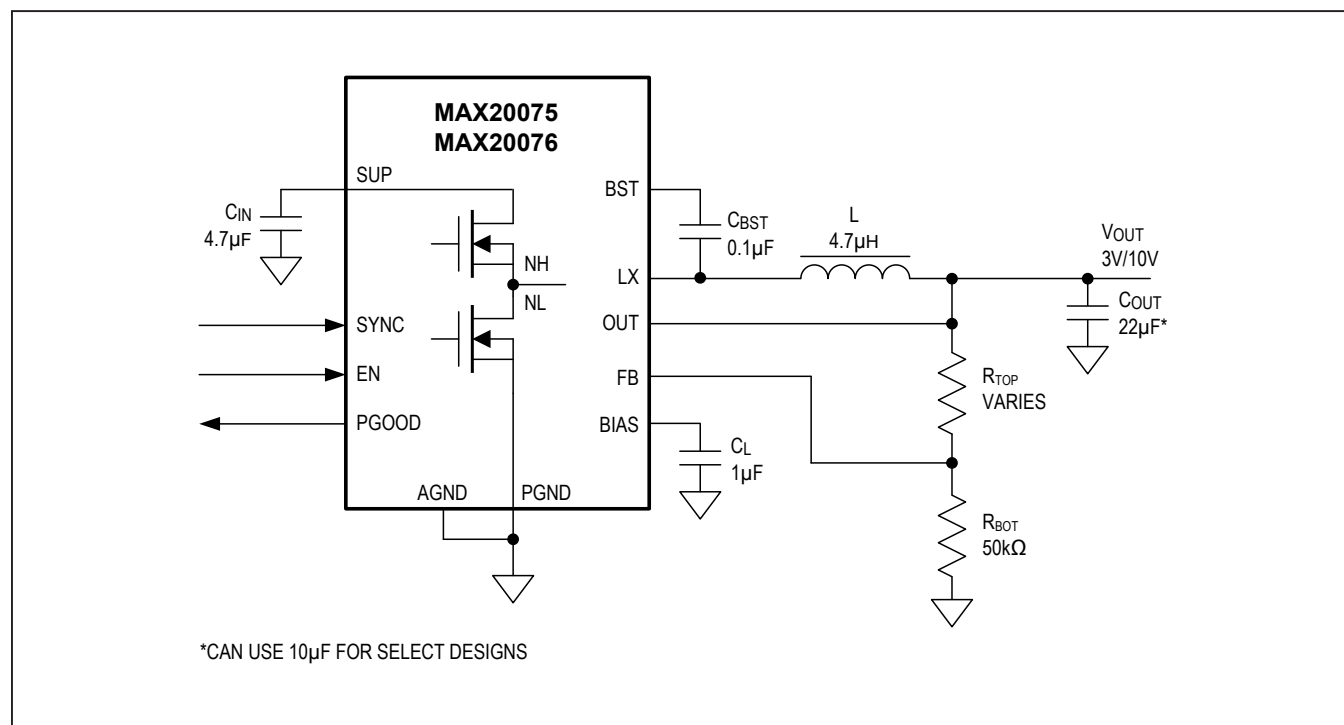
Figure 4. MAX20075/MAX20076 3V/10V Variable Output
