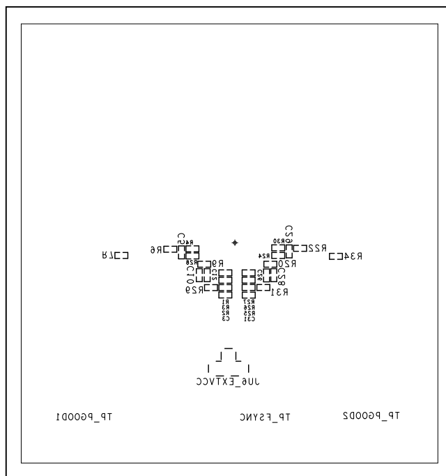
MAX20034 EV Kit Component Placement Guide—Bottom Silkscreen
