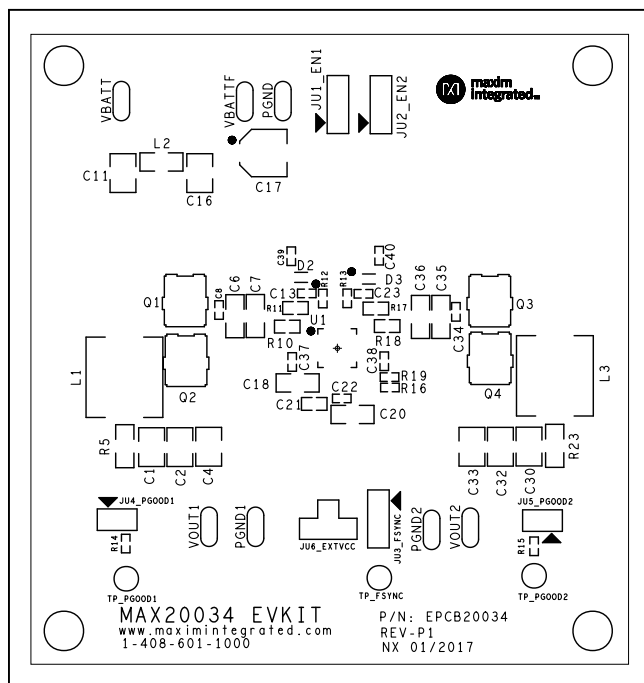
MAX20034 EV Kit Component Placement Guide—Top Silkscreen
