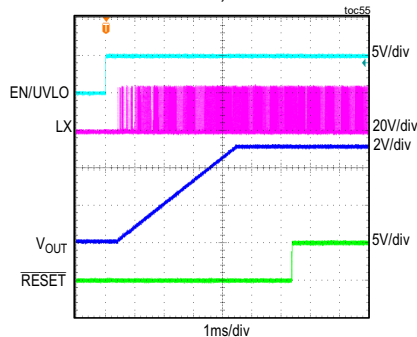
MAXM15462 STARTUP THROUGH ENABLE
