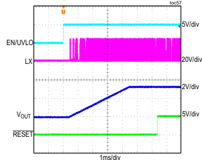
MAXM15463 STARTUP THROUGH ENABLE V_{IN} = 24V , FIXED V_{OUT} = 3.3V , FULL LOAD, PWM MODE
