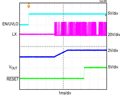
MAXM15463 STARTUP THROUGH ENABLE (2V PREBIAS) V_{IN} = 24V , FIXED V_{OUT} = 3.3V , NO LOAD, PWM MODE
