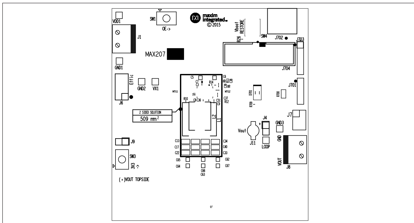
Top Silkscreen
