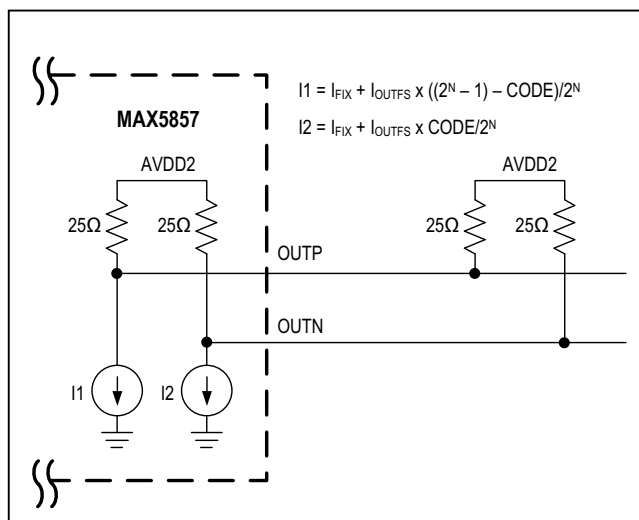
Figure 27. Output Configuration for Low Frequency Operation
