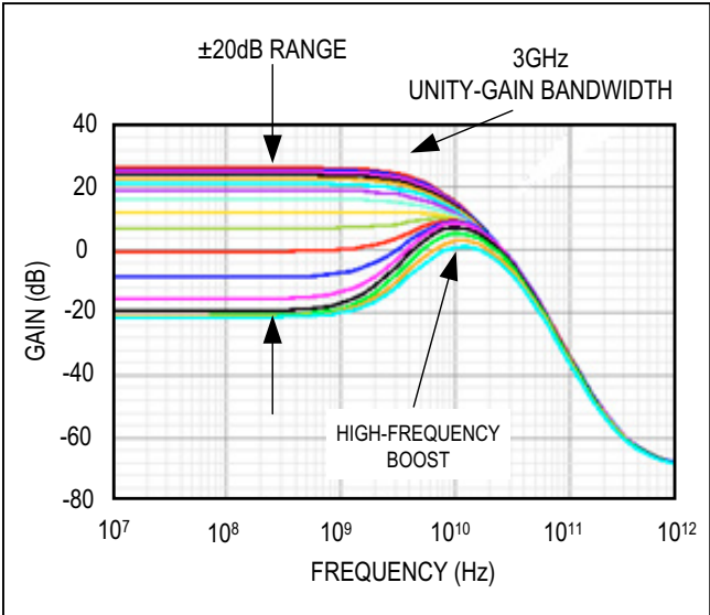
Figure 6. VGA Gain Range
