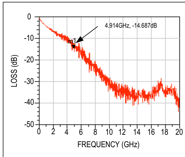
Figure 8. Channel Loss Curve (30in Nelco)
