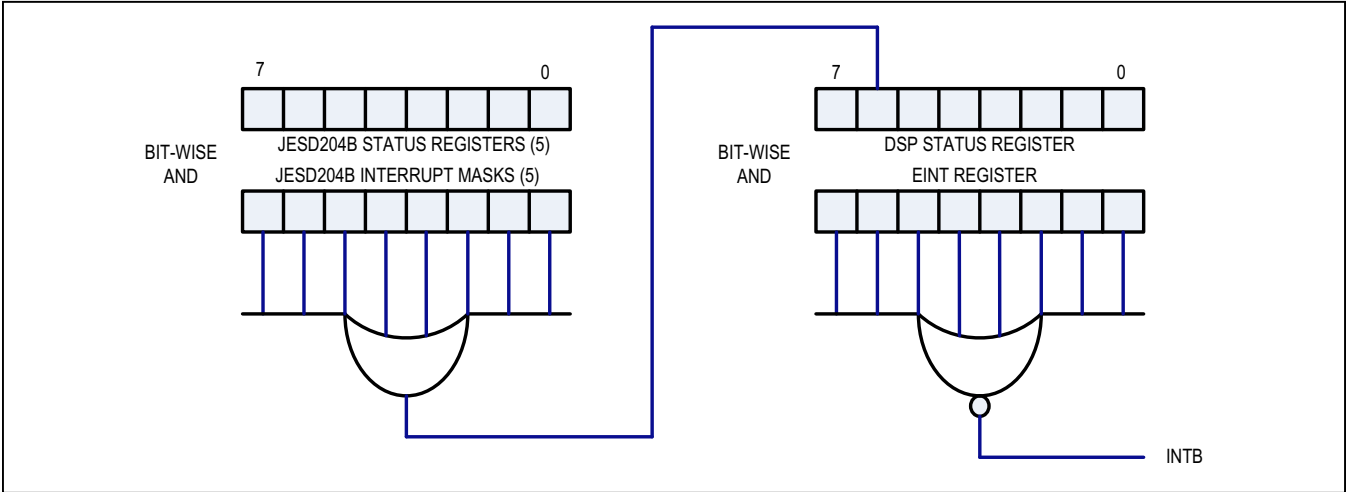
Figure 20. Interrupt Tree
