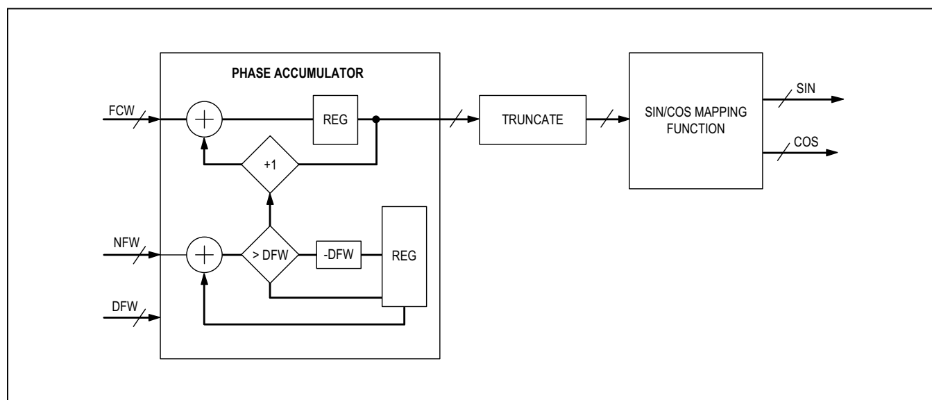
Figure 24. NCO Block Diagram
