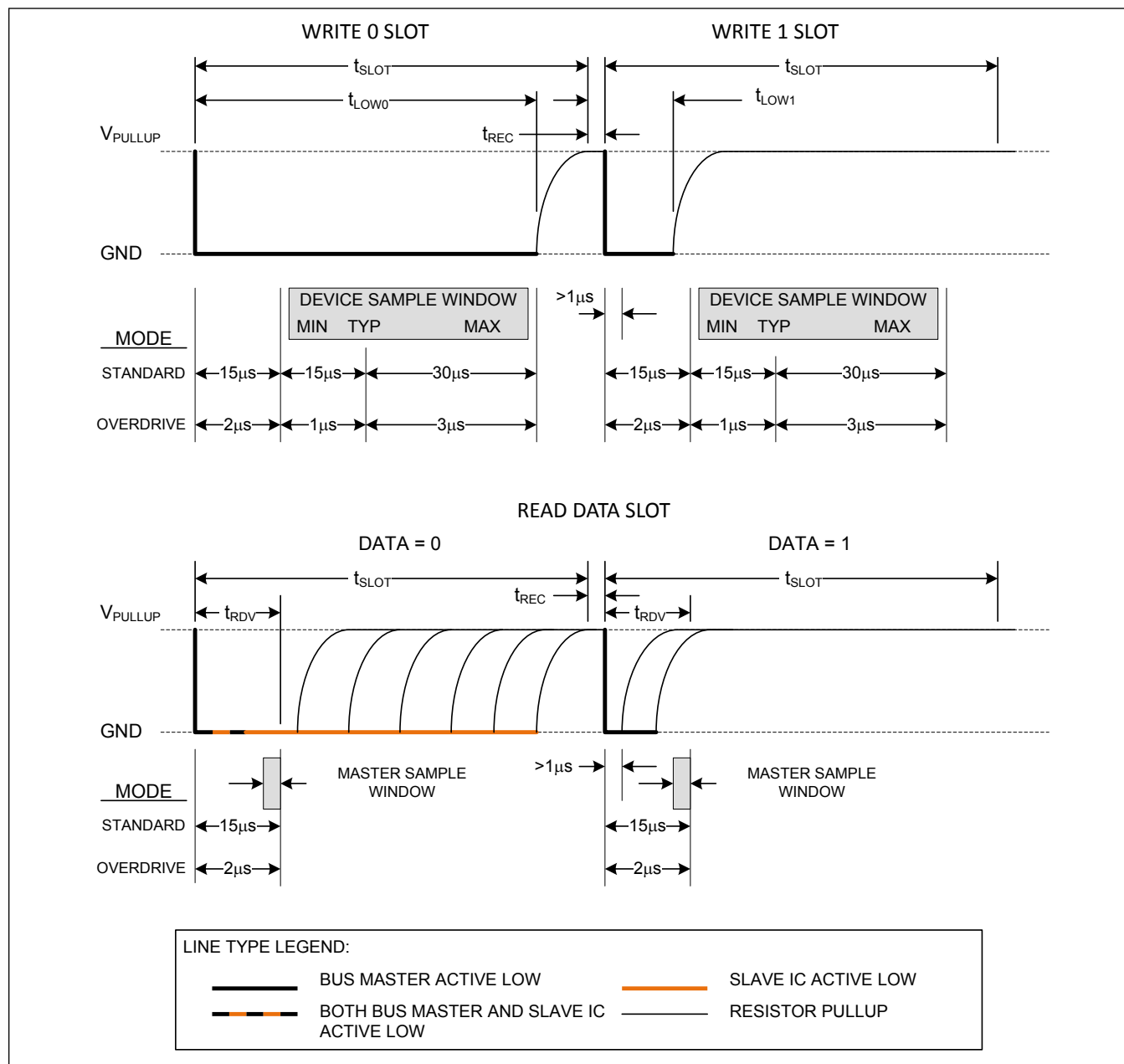
Figure 44. 1-Wire Write and Read Time Slots
