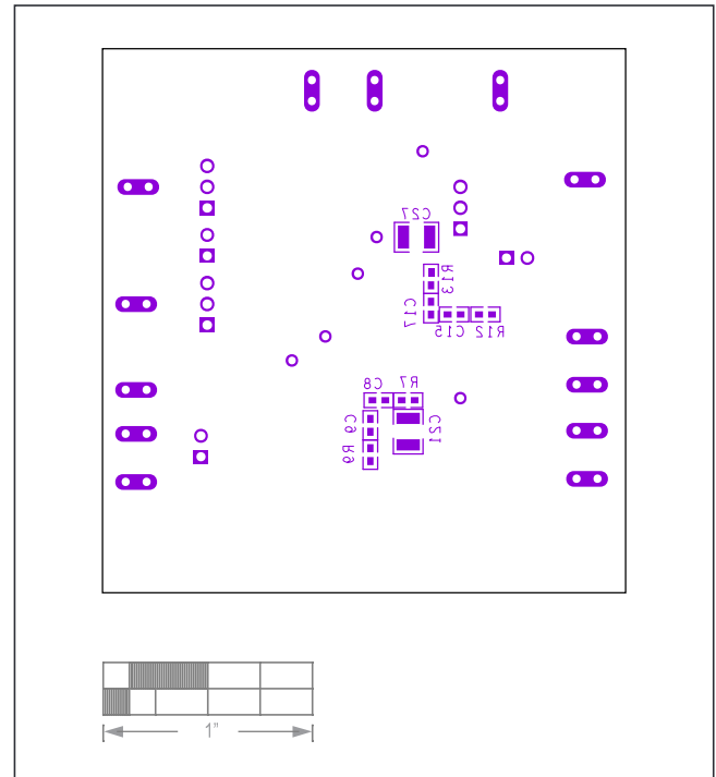
MAX25520 EV Kit PCB Layout—Bottom Silkscreen
