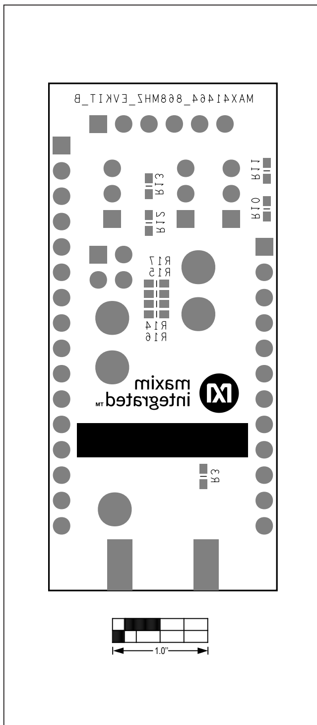
MAX4146x EV Kit PCB Layout—Bottom Silk Layer
