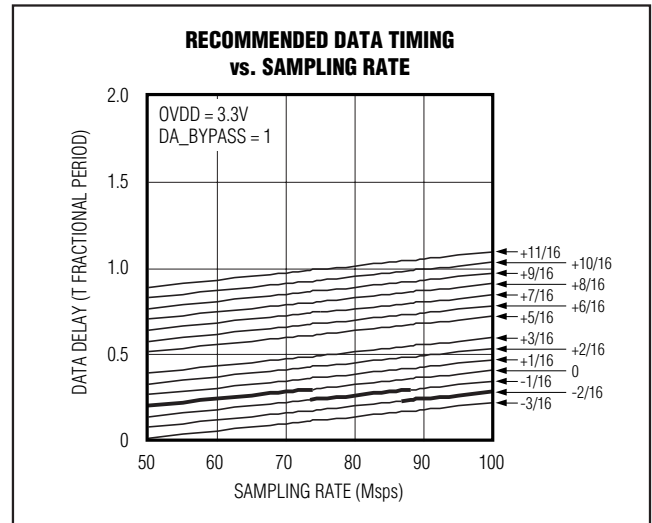
Figure 16. Recommended Data Timing ( V_{OVDD} = 3.3V )
