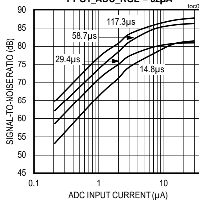
LED3 - 660nm SIGNAL-TO-NOISE RATIO vs. ADC INPUT CURRENT PPG1_ADC_RGE = 32μA
