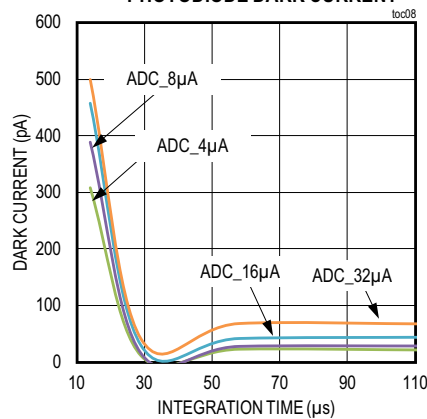
PHOTODIODE DARK CURRENT
