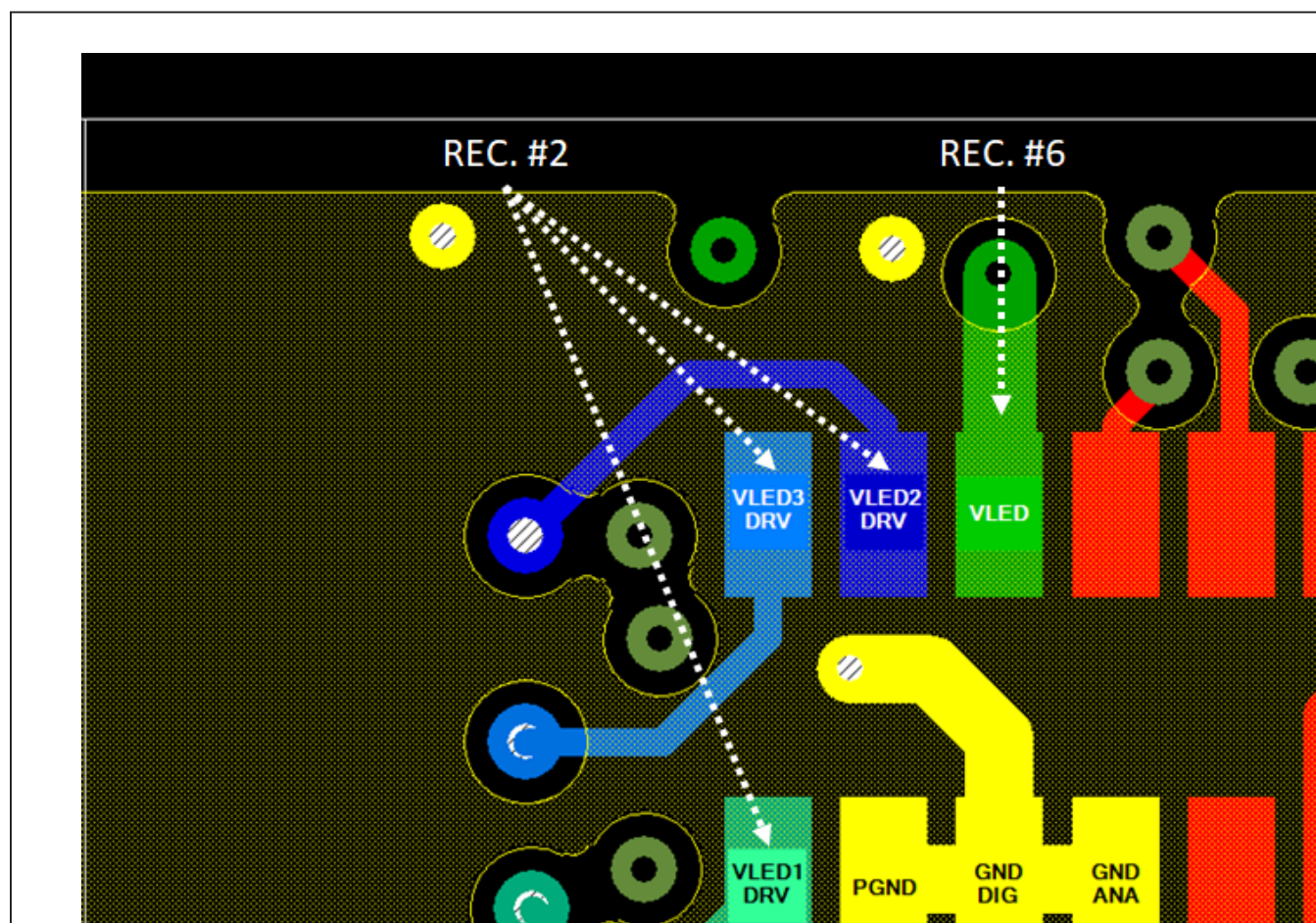
Figure 8. Layout Guideline
