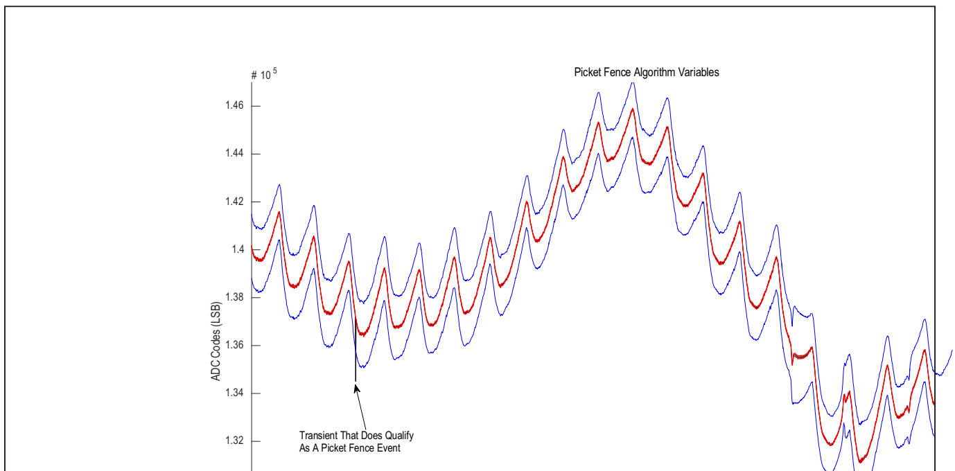
Figure 7. Picket Fences Variables In A PPG Waveform
