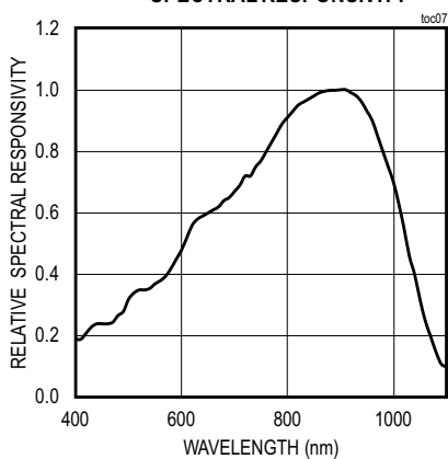
PHOTODIODE RELATIVE SPECTRAL RESPONSIVITY
