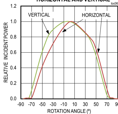
PHOTODIODE FIELD OF VIEW HORIZONTAL AND VERTICAL
