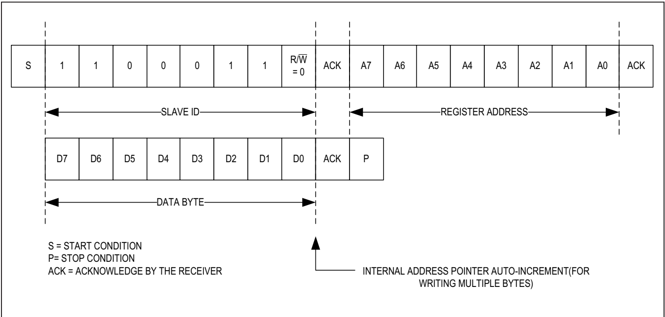
Figure 12. I 2 C Single Byte Write Transaction
