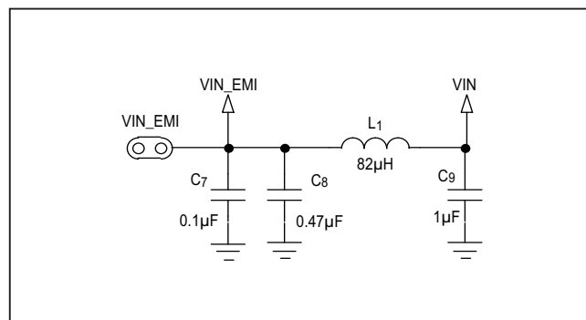
Figure 1. EMI Filter Components
