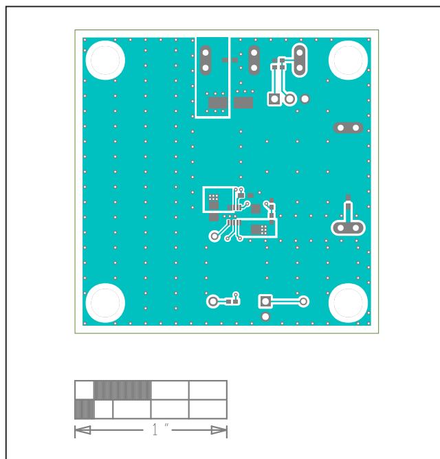
MAXM17906 EV Kit PCB Layout—Top Layer
