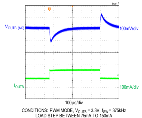
MAXM17712 LOAD TRANSIENT RESPONSE
