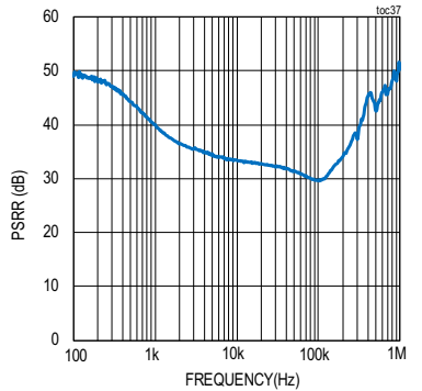
MAXM17720 POWER SUPPLY REJECTION RATIO vs. FREQUENCY
