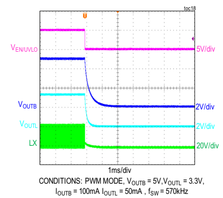
MAXM17720 SHUTDOWN THROUGH ENABLE
