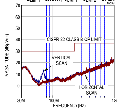
MAXM17712 RADIATED EMISSIONS PLOT L_{EMI\_1} = \text{SHORT} , C_{EMI\_1} = C_{EMI\_2} = \text{OPEN}
