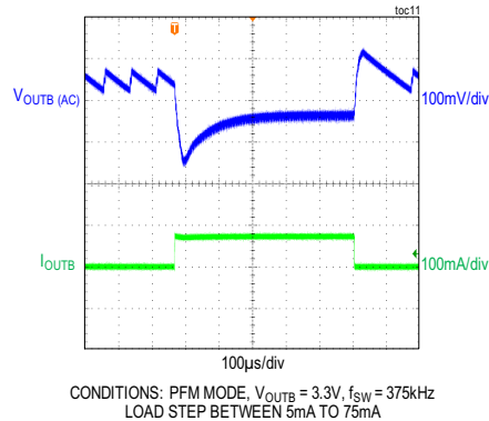
MAXM17712 LOAD TRANSIENT RESPONSE
