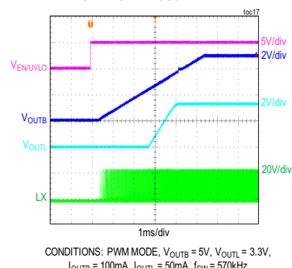
MAXM17720 STARTUP THROUGH ENABLE
