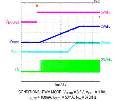
MAXM17712 STARTUP THROUGH ENABLE
