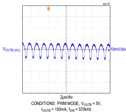
MAXM17720, MAXM17724 OUTPUT VOLTAGE RIPPLE
