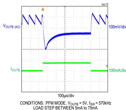
MAXM17720, MAXM17724 LOAD TRANSIENT RESPONSE
