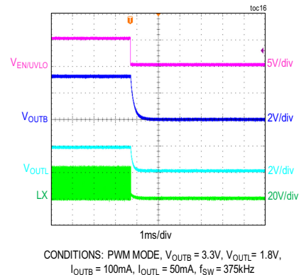
MAXM17712 SHUTDOWN THROUGH ENABLE
