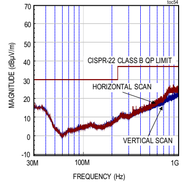
MAXM17633 RADIATED EMISSIONS PLOT V_{OUT} = 3.3V , f_{SW} = 800kHz , FULL LOAD, PWM MODE
