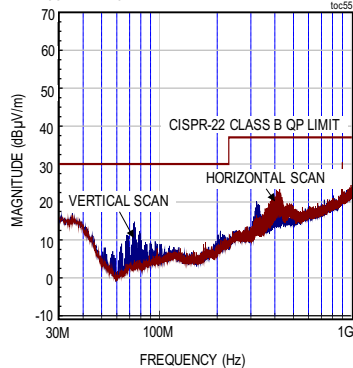
MAXM17634 RADIATED EMISSIONS PLOT V_{OUT} = 5V , f_{SW} = 1MHz , FULL LOAD, PWM MODE
