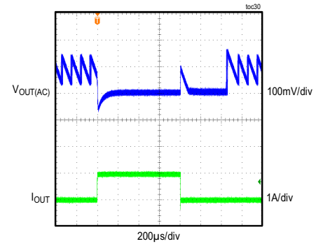
MAXM17633 LOAD-TRANSIENT RESPONSE V_{OUT} = 3.3V , f_{SW} = 800kHz , PFM MODE, LOAD CURRENT STEPPED FROM 20mA TO 1A
