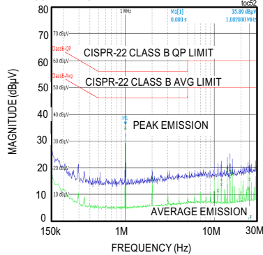
MAXM17634 CONDUCTED EMISSIONS PLOT V_{OUT} = 5V , f_{SW} = 1MHz , FULL LOAD, PWM MODE
