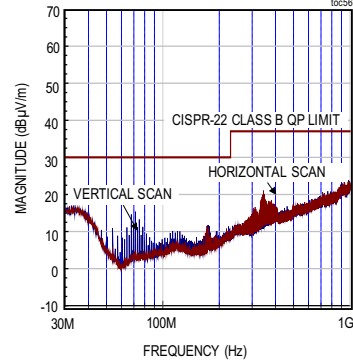
MAXM17635 RADIATED EMISSIONS PLOT V_{OUT} = 12V , f_{SW} = 1.8MHz , FULL LOAD, PWM MODE
