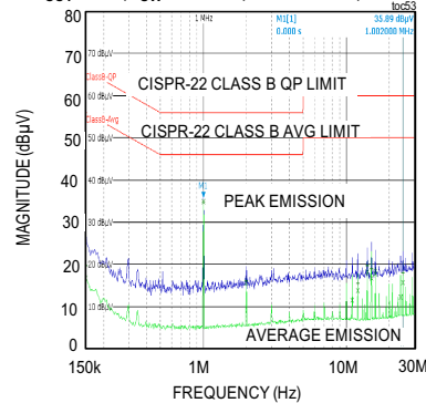
MAXM17635 CONDUCTED EMISSIONS PLOT V_{OUT} = 12V , f_{SW} = 1.8MHz , FULL LOAD, PWM MODE
