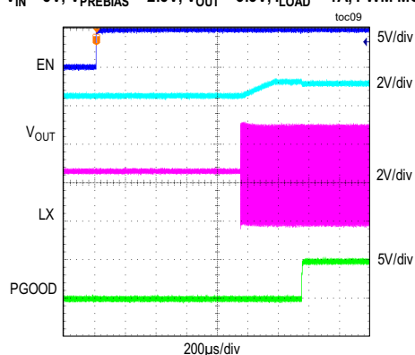
MAXM17624 STARTUP INTO PREBIAS V_{IN} = 5V , V_{PREBIAS} = 2.5V , V_{OUT} = 3.3V , I_{LOAD} = 1A , PWM MODE
