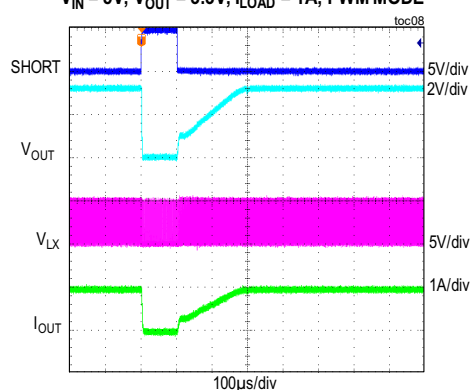
MAXM17624 TEMPORARY OUTPUT SHORT V_{IN} = 5V , V_{OUT} = 3.3V , I_{LOAD} = 1A , PWM MODE
