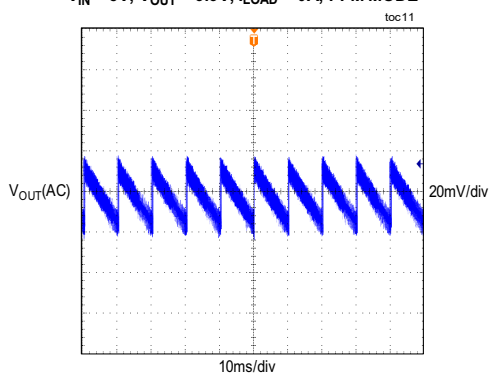
MAXM17624 OUTPUT VOLTAGE RIPPLE V_{IN} = 5V , V_{OUT} = 3.3V , I_{LOAD} = 0A , PFM MODE
