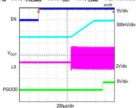
MAXM17623 STARTUP INTO PREBIAS V_{IN} = 3.3V , V_{PREBIAS} = 0.8V , V_{OUT} = 1.5V , I_{LOAD} = 1A , PWM MODE
