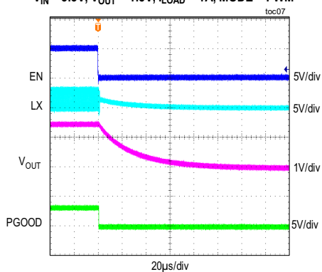
MAXM17623 SHUTDOWN THROUGH ENABLE V_{IN} = 3.3V , V_{OUT} = 1.5V , I_{LOAD} = 1A , MODE = PWM
