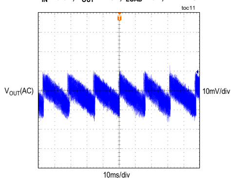
MAXM17623 OUTPUT VOLTAGE RIPPLE V_{IN} = 3.3V , V_{OUT} = 1.5V , I_{LOAD} = 0A , PFM MODE
