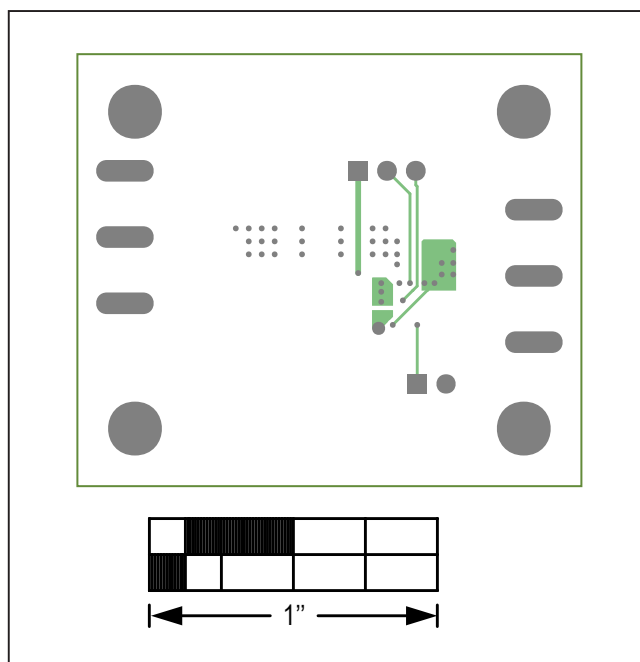
MAXM17623 EV Kit PCB Layout—Layer 3 Power
