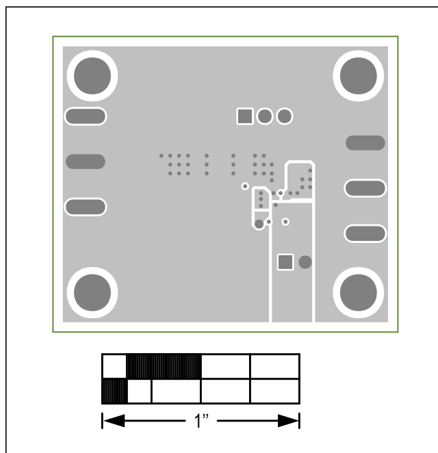
MAXM17623 EV Kit PCB Layout—Layer 2 Ground
