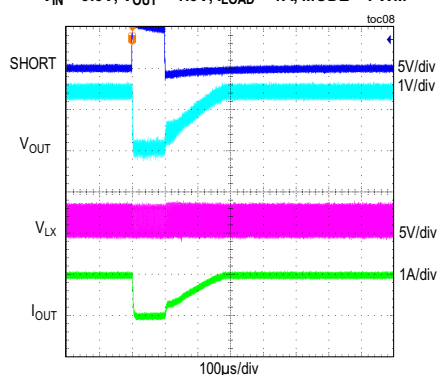
MAXM17623 TEMPORARY OUTPUT SHORT V_{IN} = 3.3V , V_{OUT} = 1.5V , I_{LOAD} = 1A , MODE = PWM
