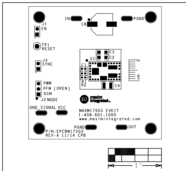
Figure 1 MAXM17503 EV Kit Component Placement Guide— Component Side
