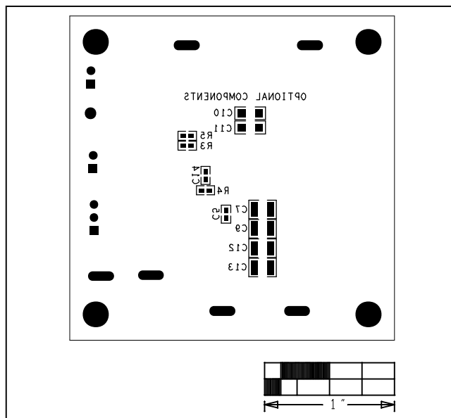
Figure 2 MAXM17503 EV Kit Component Placement Guide— Solder Side
