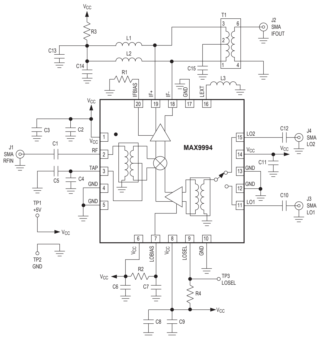
Figure 2. MAX9994 EV Kit Schematic
