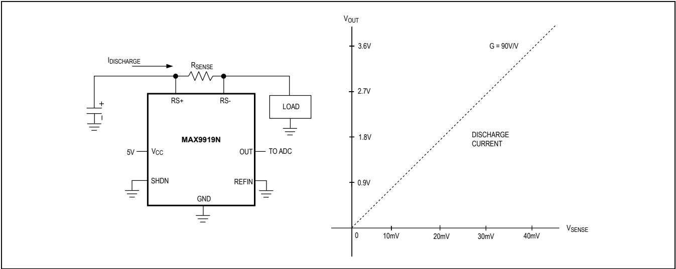
Figure 1. Unidirectional Operation
