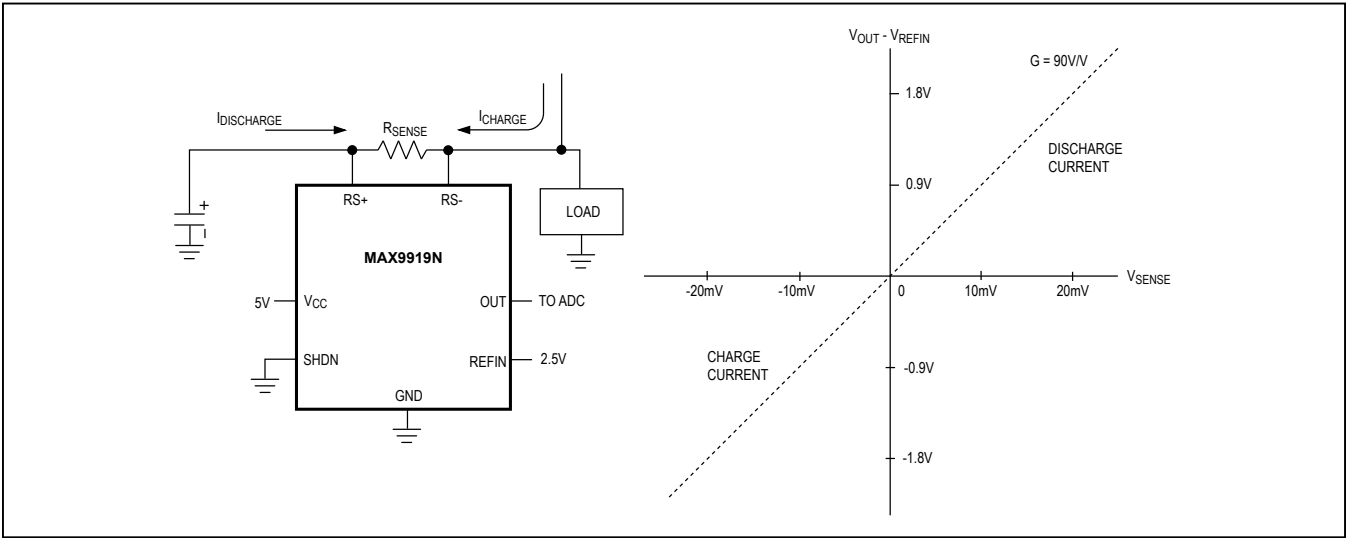
Figure 2. Bidirectional Operation
