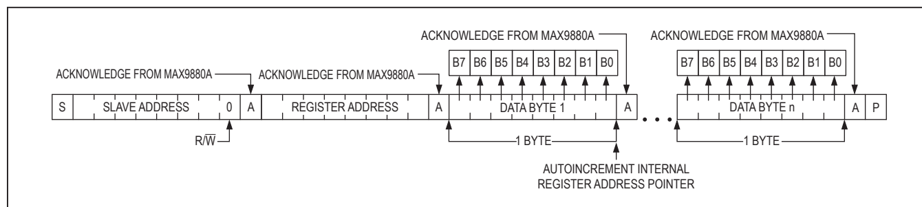
Figure 18. Writing n Bytes of Data
