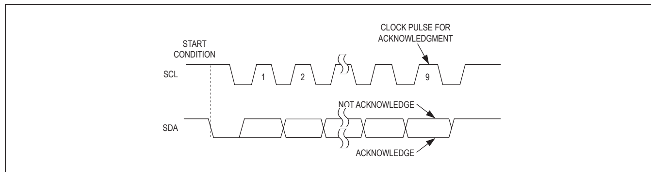
Figure 16. Acknowledge
