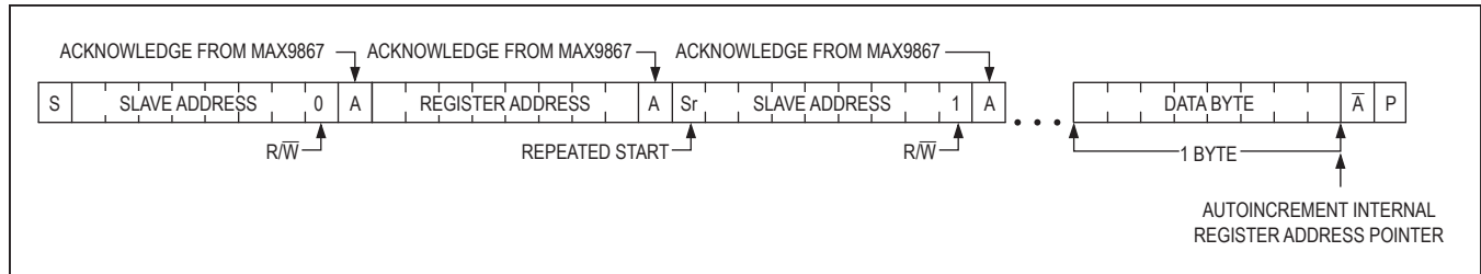
Figure 15. Reading n Bytes of Data from the MAX9867
