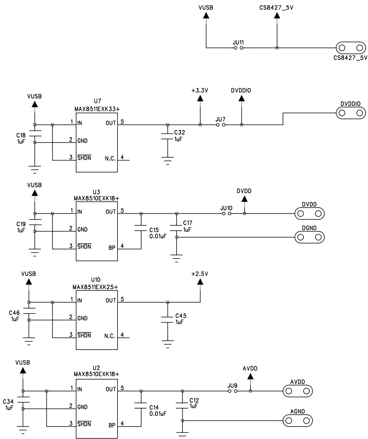
Figure 9e. MAX9860 EV Kit Schematic (Sheet 5 of 5)
