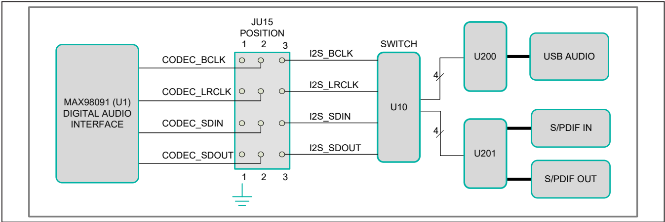
Figure 12. I²S Routing
