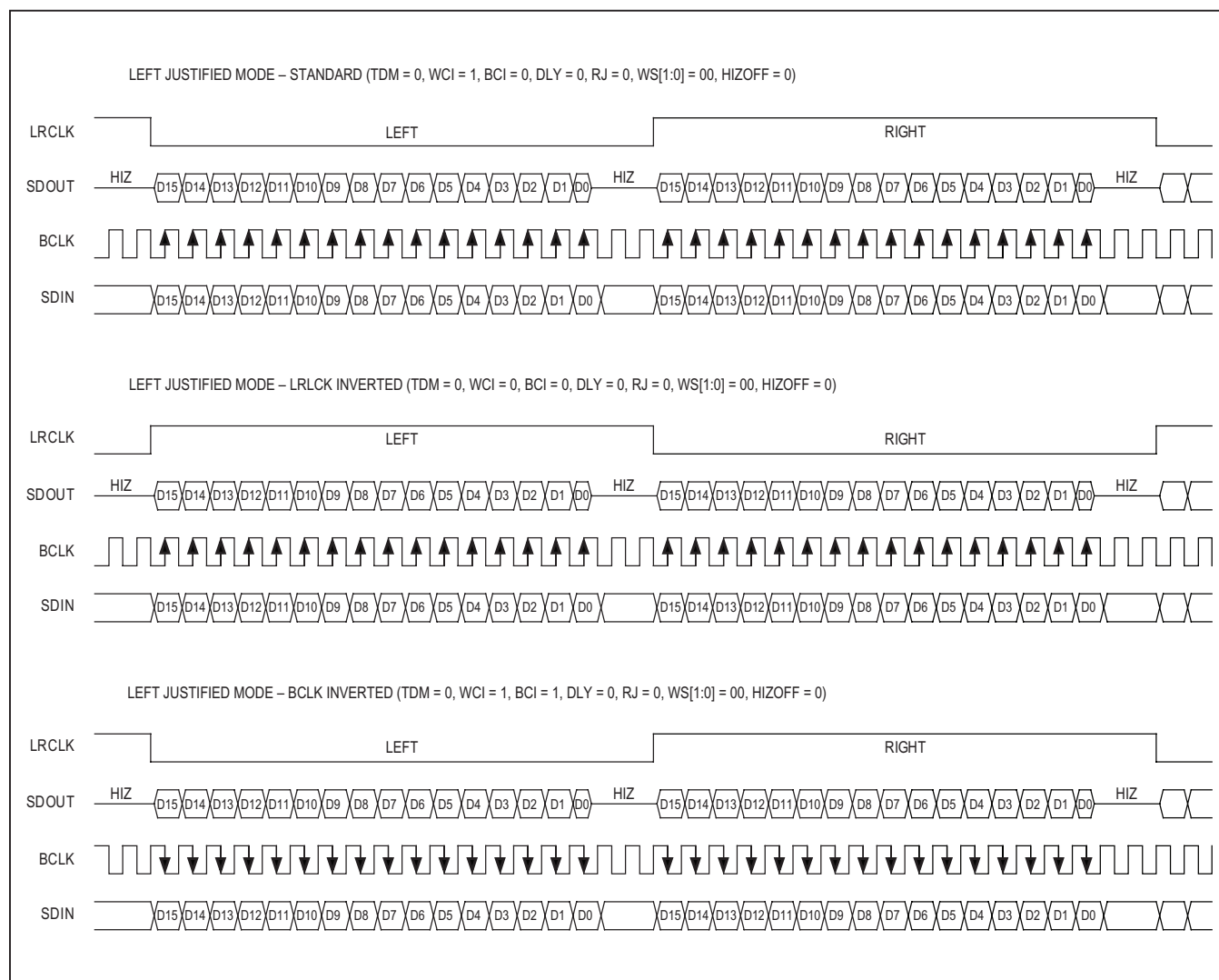
Figure 21. DAI Timing for Left Justified Data Formats
