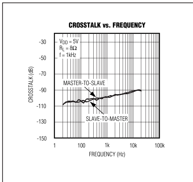
Figure 4. Master-Slave Crosstalk
