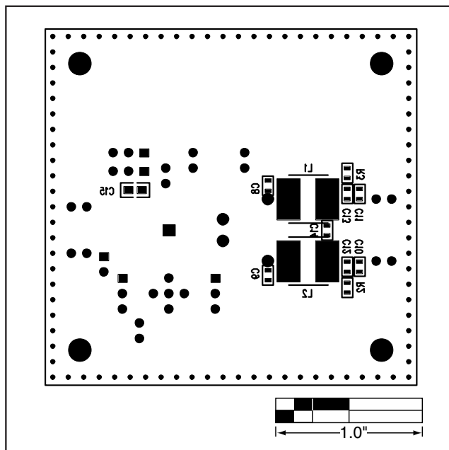
Figure 9. MAX9759 EV Kit Component Placement Guide—Solder Side
