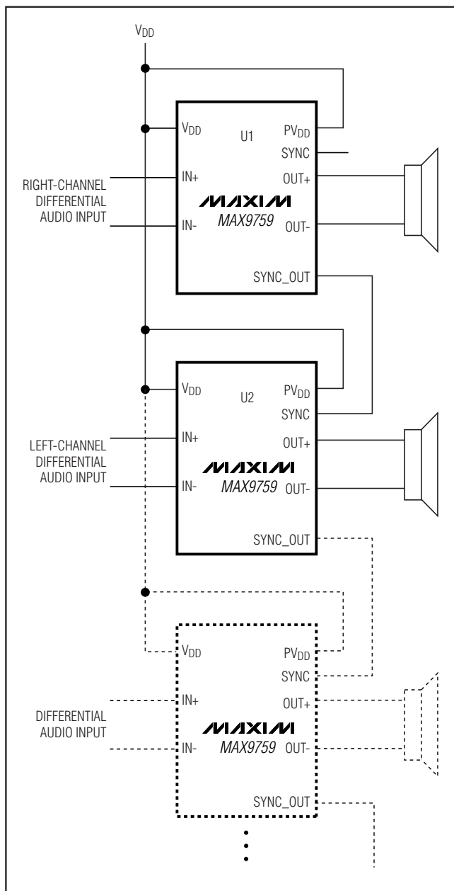
Figure 2. Master-Slave Configuration
