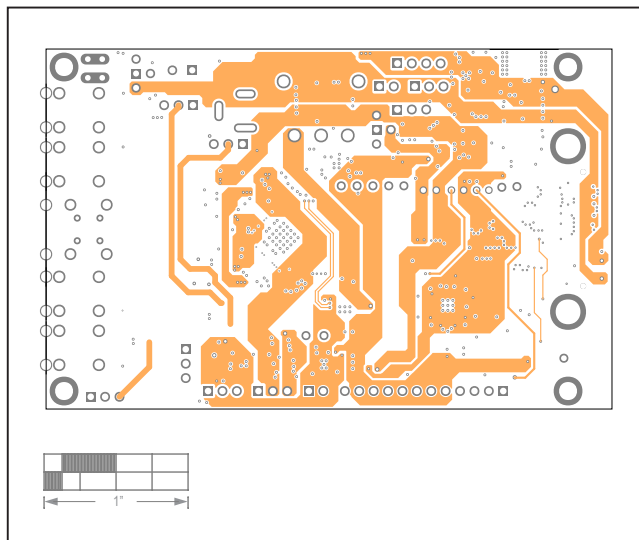
MAX96724 EV Kit—Layer5
