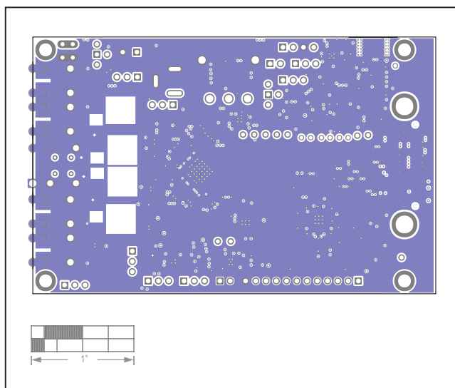
MAX96724 EV Kit—Layer7
