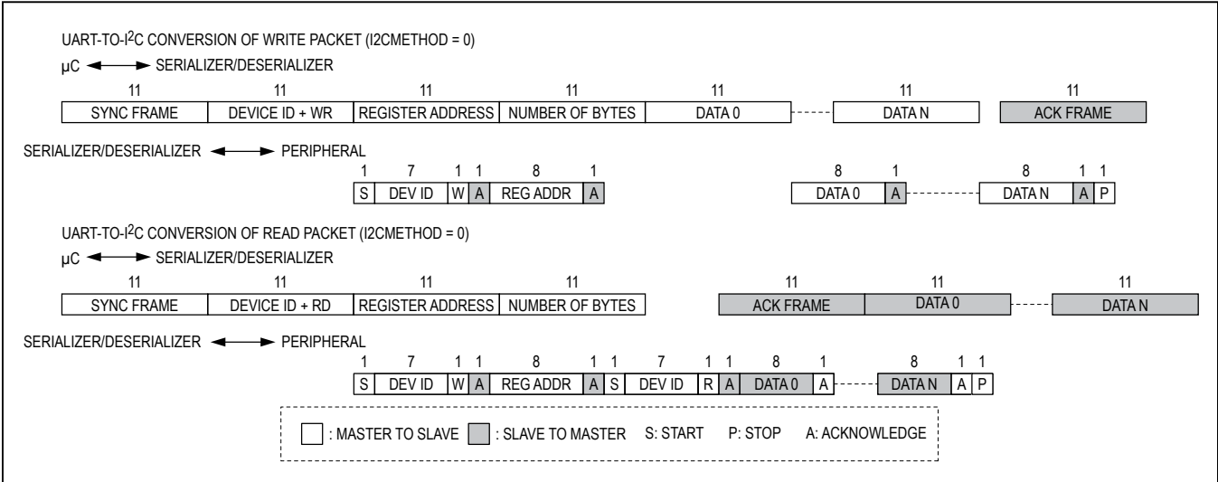
Figure 26. Format Conversion Between GMSL UART and I 2 C with Register Address (I2CMETHOD = 0)
