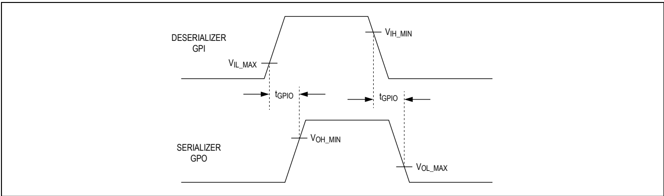
Figure 10. GPI-to-GPO Delay
