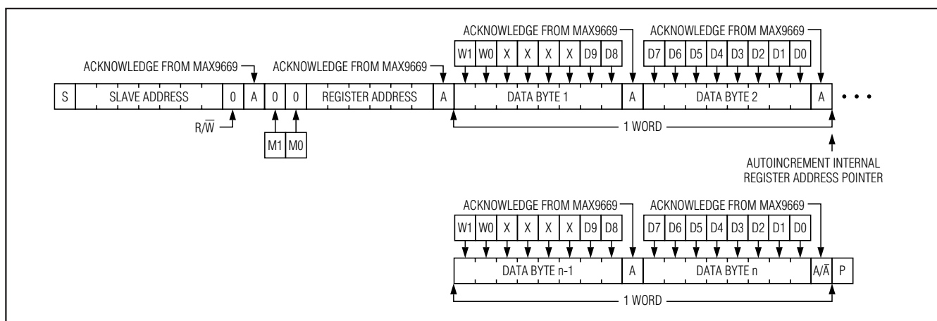
Figure 5. Writing n Bytes of Data to the MAX9669
