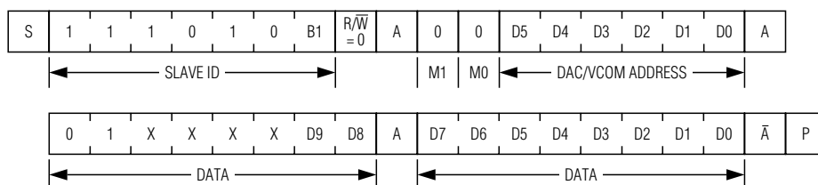
Figure 10. Single MTP Programming
