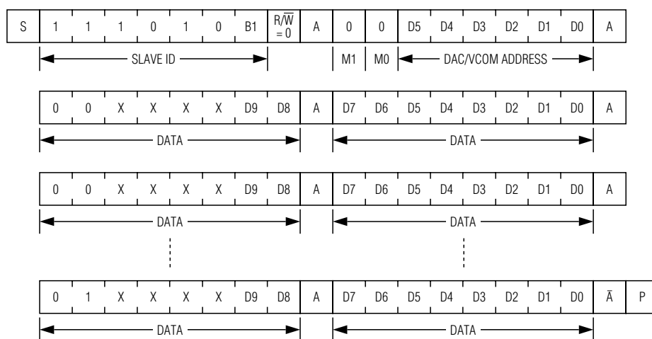
Figure 11. Multiple MTP Programming
