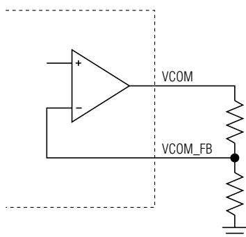
Figure 15. VCOM Operational Amplifier with Feedback Resistors
