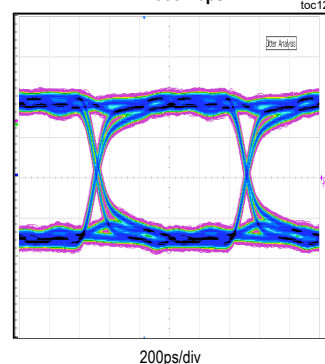
MIPI DATA EYE PATTERN 1000Mbps
