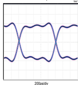
MIPI CLOCK EYE PATTERN 1000Mbps
