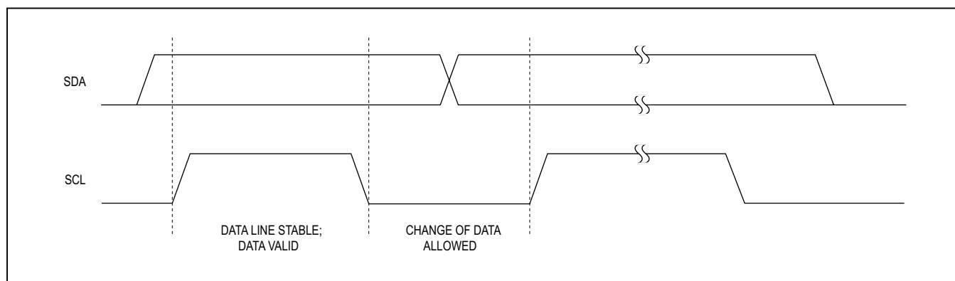
Figure 30. Bit Transfer
