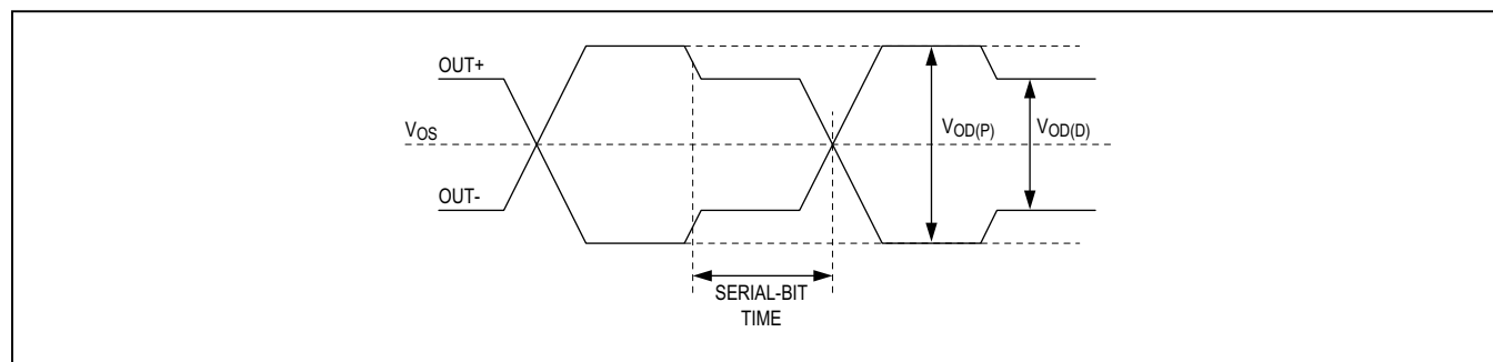
Figure 2. Output Waveforms at OUT+ , OUT-
