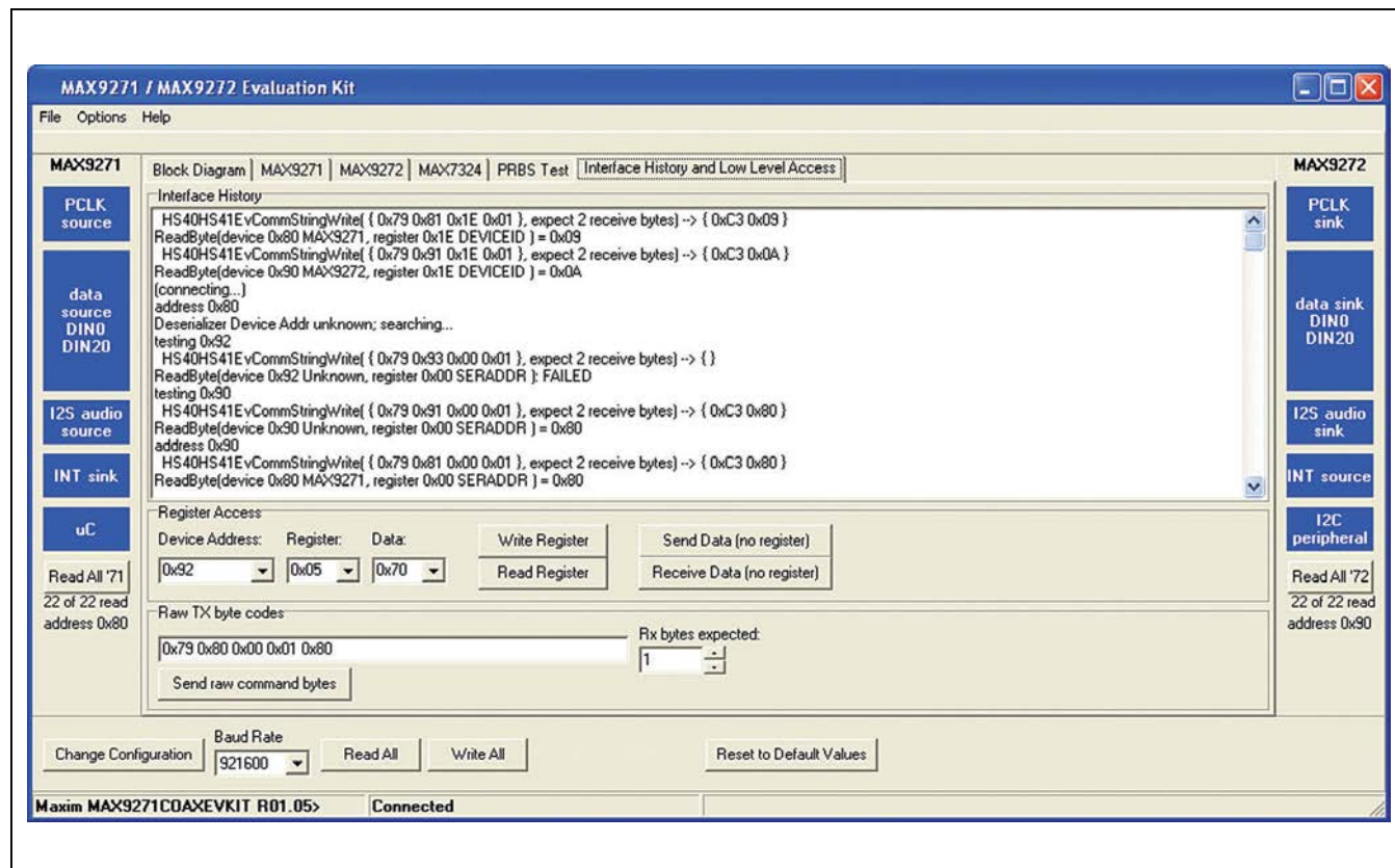
Figure 6. MAX9271 EV Kit Software Main Window (Interface History and Low Level Access Tab)
