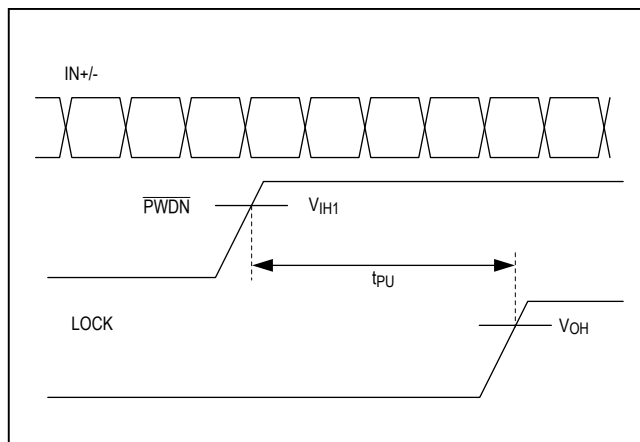
Figure 12. Power-Up Delay
