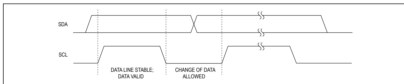
Figure 25. Bit Transfer
