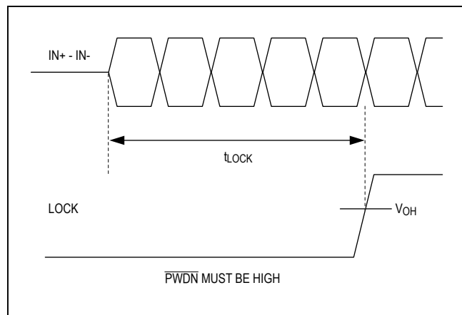
Figure 11. Lock Time
