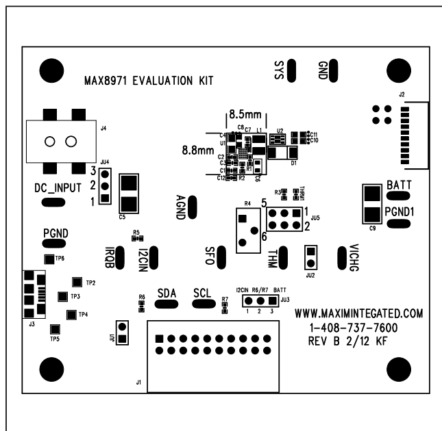
MAX9971 EV Kit Component Placement Guide—Component Side
