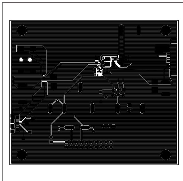
MAX8971 EV Kit PCB Layout—Component Side
