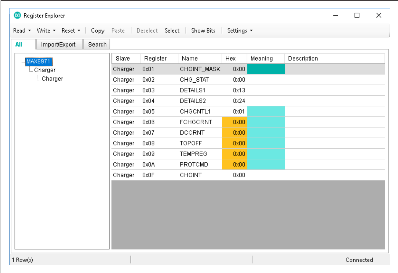
Figure 5. MAX8971 Register Explorer
