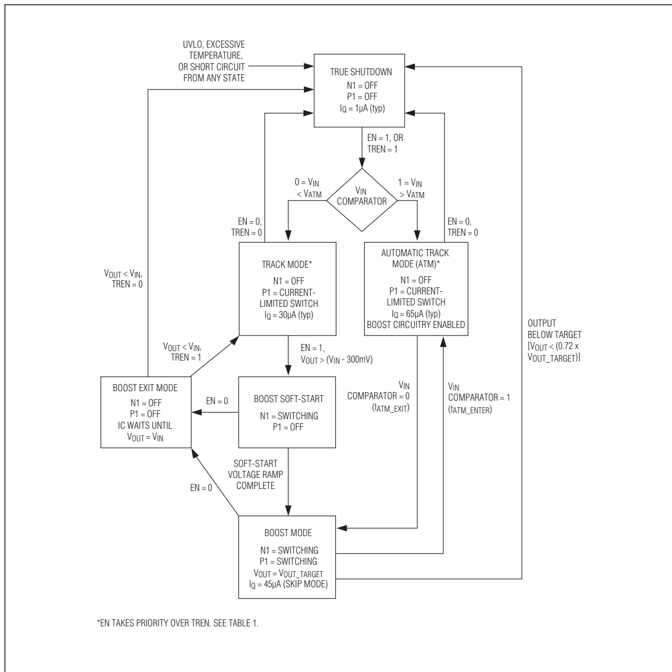
Figure 2. State Diagram
