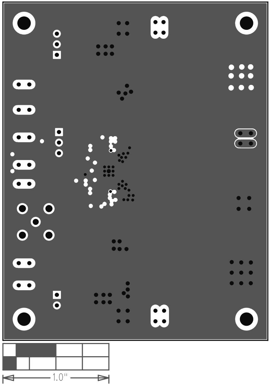
Figure 5. MAX8855 EV Kit PCB Layout—Layer 3
