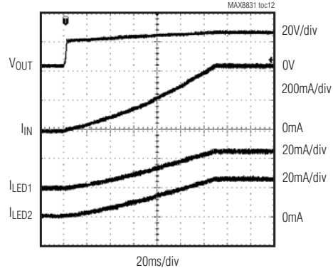
SOFT-START RESPONSE
