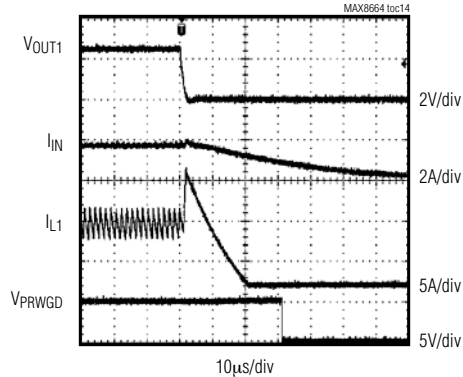
SHORT-CIRCUIT WAVEFORMS
