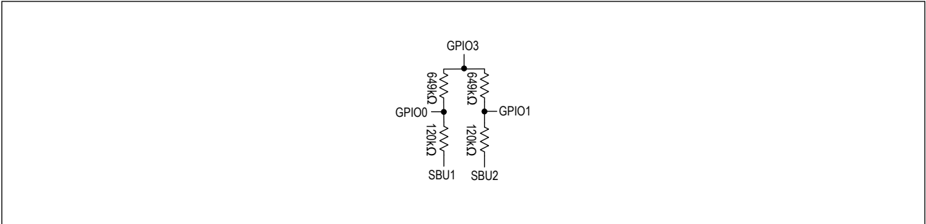
Figure 3. SBU Configuration
