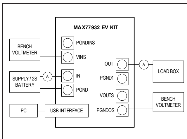
Figure 1. MAX77932 EV Kit Board Connections
