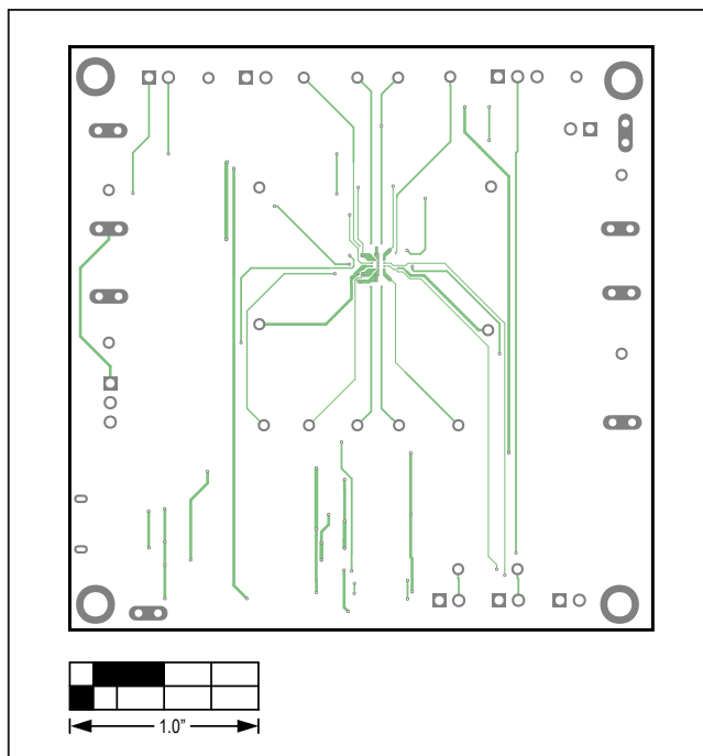
MAX77932 EV Kit PCB Layout—Layer 3
