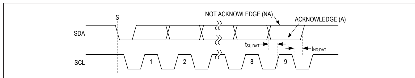
Figure 5. Acknowledge Bit
