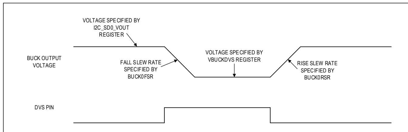
Figure 1. DVS Functionality
