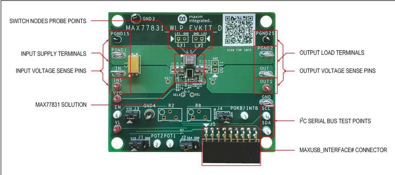
Figure 2. MAX77831 EV Kit Photo
