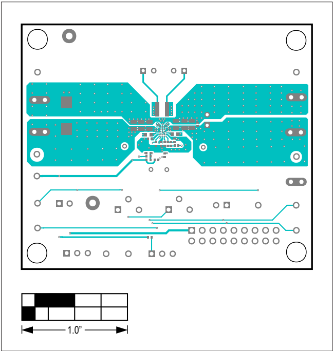
MAX77831 EV Kit PCB Layout — Top View
