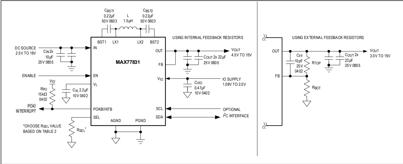
Figure 1. Application Circuit for MAX77831
