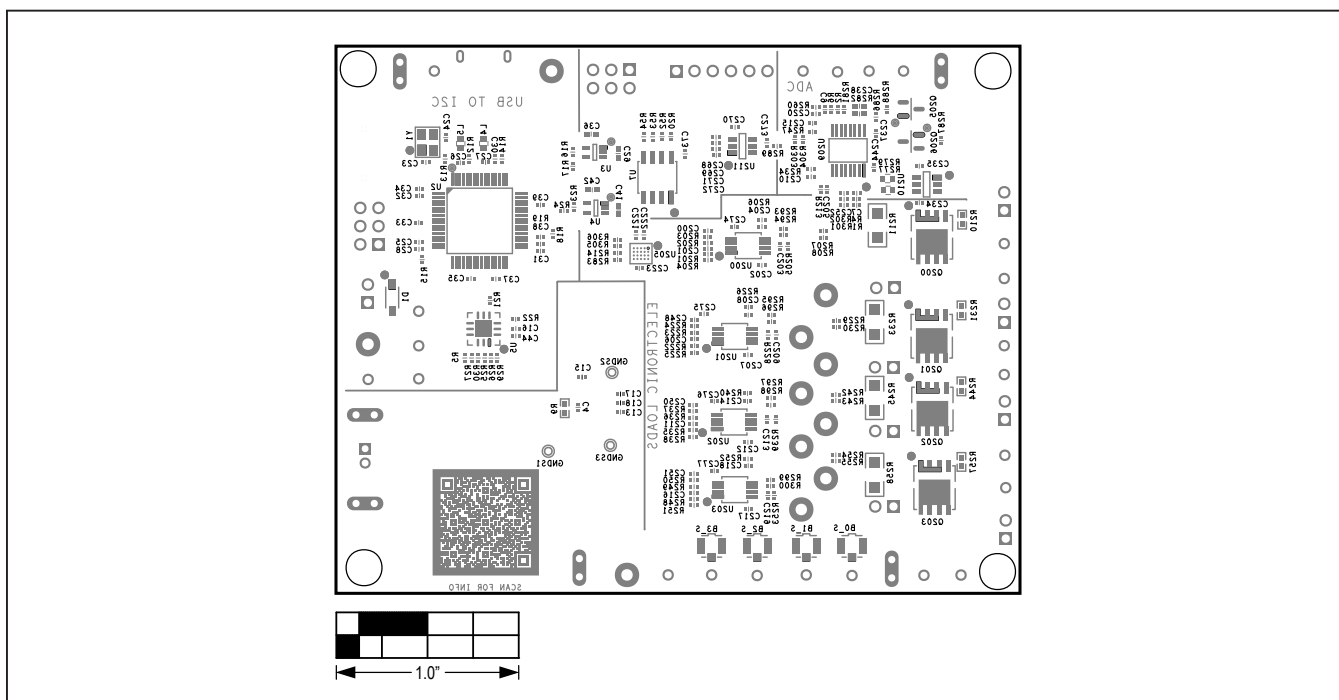
MAX77655 EV Kit PCB Layout – Silkscreen Bottom
