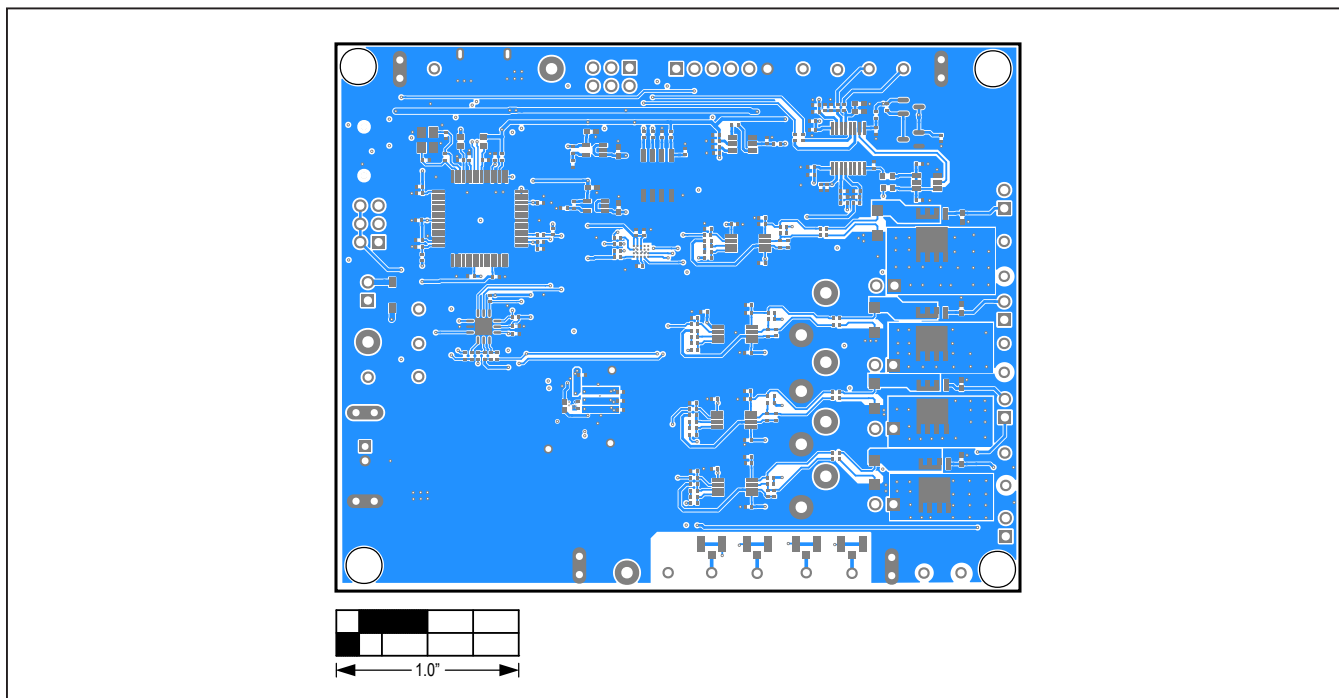
MAX77655 EV Kit PCB Layout – Bottom Layer
