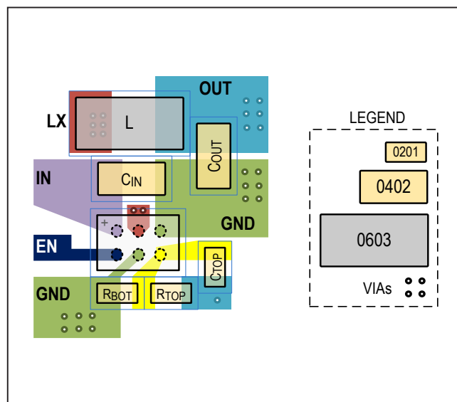
Figure 2. Example Layout
